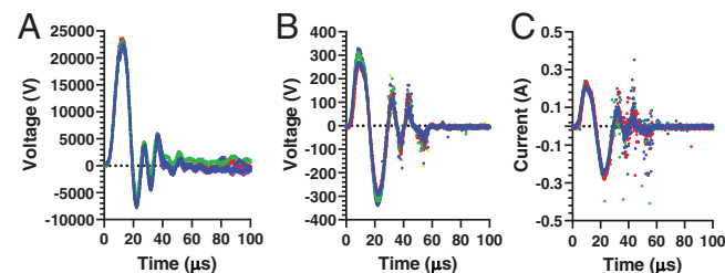
Fig. 2. Representative electrical output profiles for piezoelectric pulser used for electroporation. Piezoelectric pulser activated by open-circuit measurements made (A) by connecting the pulser leads to the oscilloscope (voltage profile) and (B and C) by pulsing in porcine skin ex vivo (B, voltage profile; C, current profile). Multiple replicate voltage and current profiles are shown ( n = 4 to 6).
